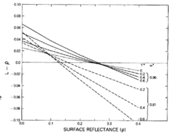
Figure 5 A figure from Fraser and Kaufmann, 1985. Fraser, R.S.; Kaufman, Y.J. The relative importance of aerosol scattering and absorption in remote sensing. IEEE Trans. Geosci. Remote Sens. 1985 , GE-23, 625–633.
